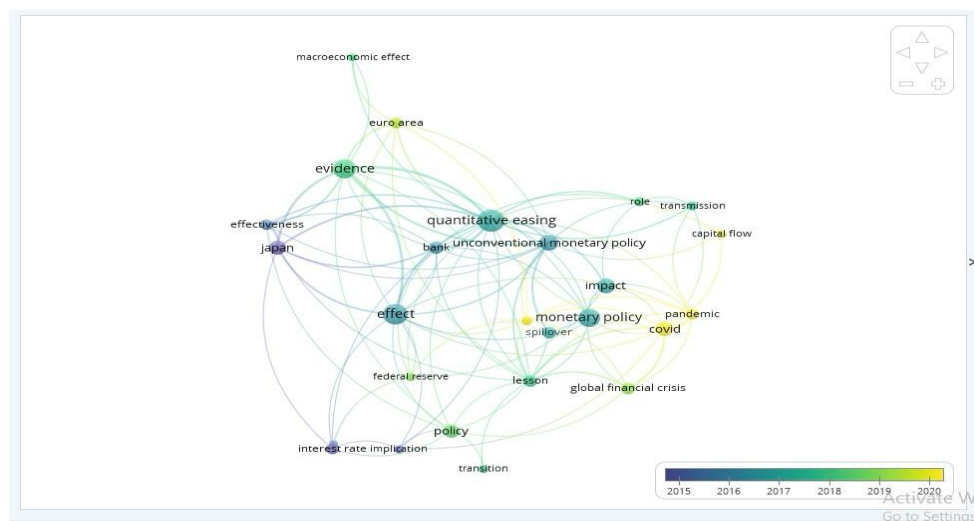
Gambar 1. Analisis VOSViewer
